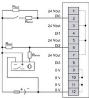
2-wire or 3-wire connection (Sink inputs with the external power supply)
